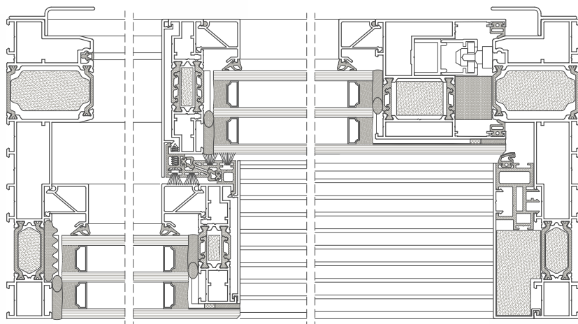
PJŪVIS PER DP 180 PRIMEVIEW GLASS DURIS
