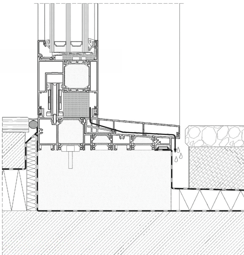
PJŪVIS PER DP 180 PRIMEVIEW GLASS DURIS
