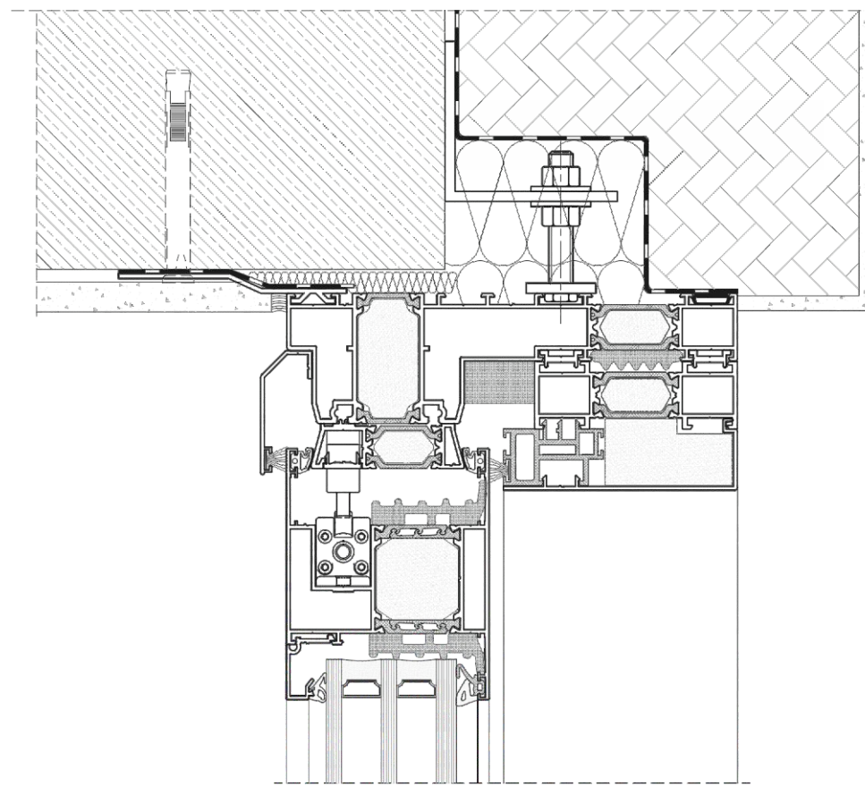
PJŪVIS PER DP 180 PRIMEVIEW DURIS FASADE
