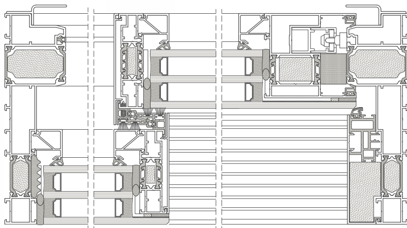
PRIEREZ DVERAMI DP180 PRIMEVIEW GLASS
