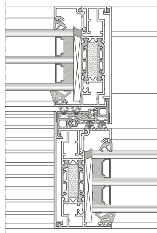
PRIEREZ STĽPIKOM DP 180 PRIMEVIEW
