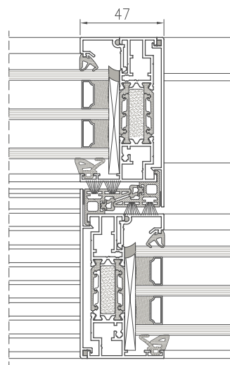
CROSS-SECTION THROUGH A NARROW POST DP 180 PRIMEVIEW
