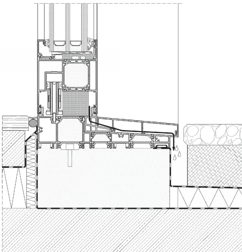
DP 180 PRIMEVIEW BOTTOM SECTION
