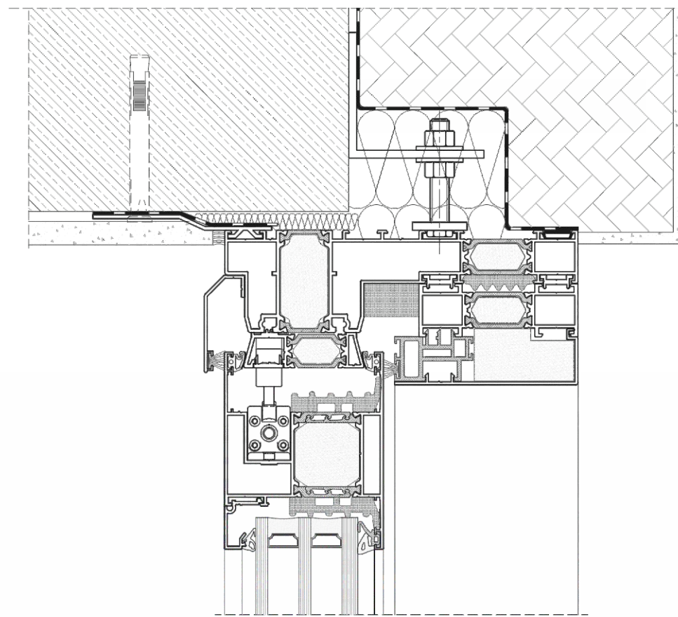
DP 180 PRIMEVIEW TOP SECTION
