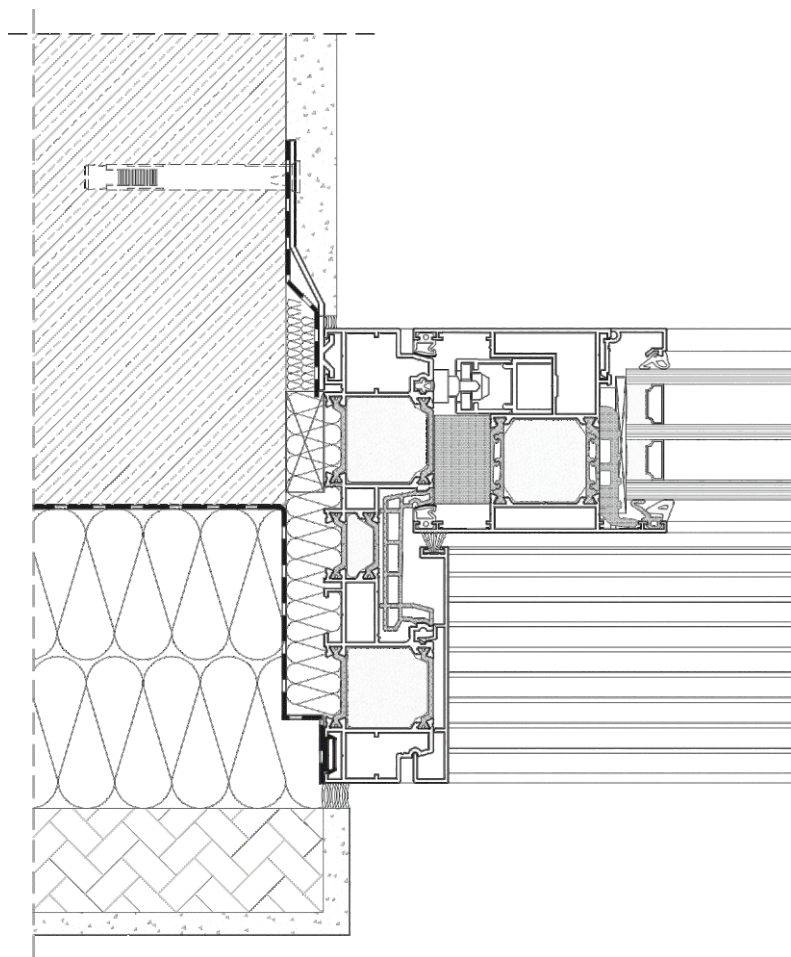
DP 180 PRIMEVIEW - LATERAL CROSS-SECTIONY
